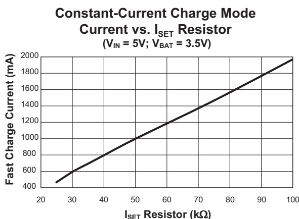
Figure 3: Constant-Current Mode Charge I_{CH\_CC} Setting vs. I_{SET} Resistor.
