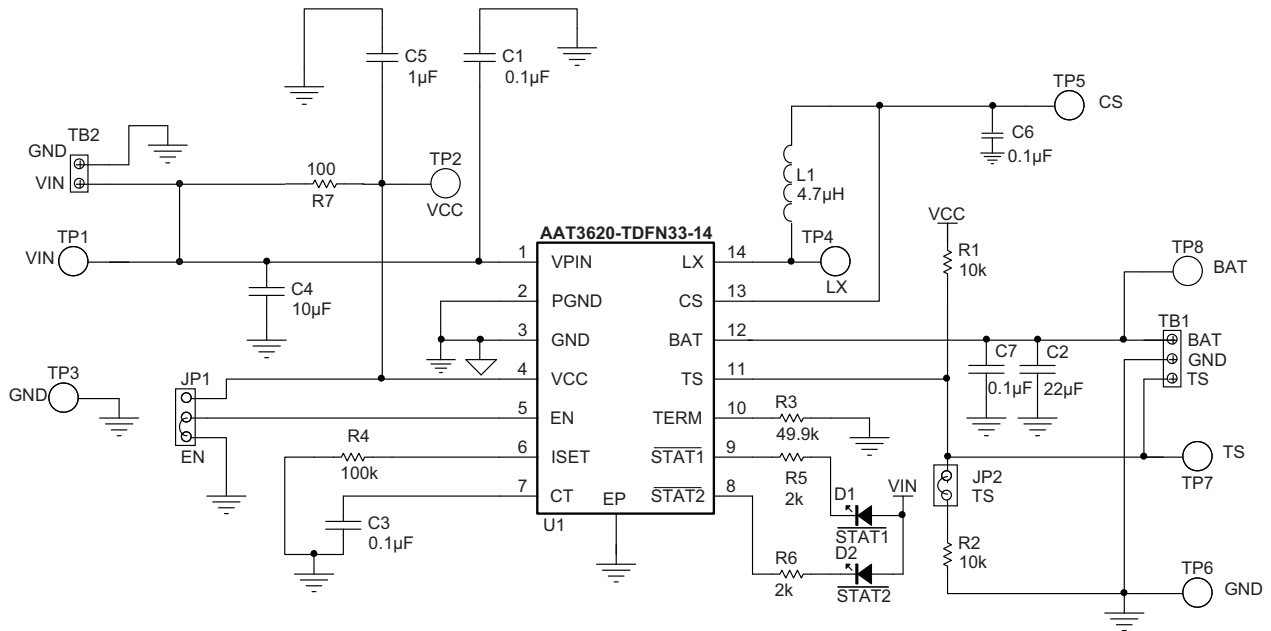
Figure 5: AAT3620 2A Evaluation Board Schematic.
