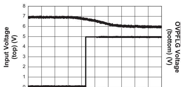
OVPFLG Release Delay Time ( R_{LOAD} = 100\Omega , OVP Trip Point 6.75V)
