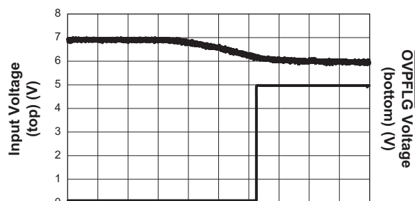
OVPFLG Release Delay Time ( R_{LOAD} = 100\Omega , OVP Trip Point 6.25V)
