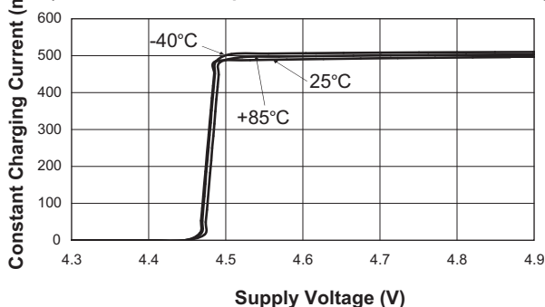
Constant Charging Current vs. Supply Voltage (USBH; CHRUSB = Open; V BAT = 3.6V; USBSET = 71.5k \Omega )
