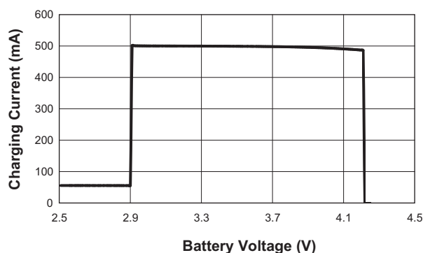
Charging Current vs. Battery Voltage (USBH; USBSET = 71.5k \Omega )
