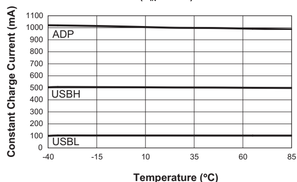
Constant Charge Current vs. Temperature ( V_{IN} = 5.0V)
