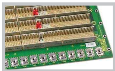
Power Nuts
