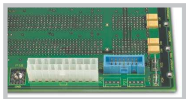
ATX & Utility Connectors
