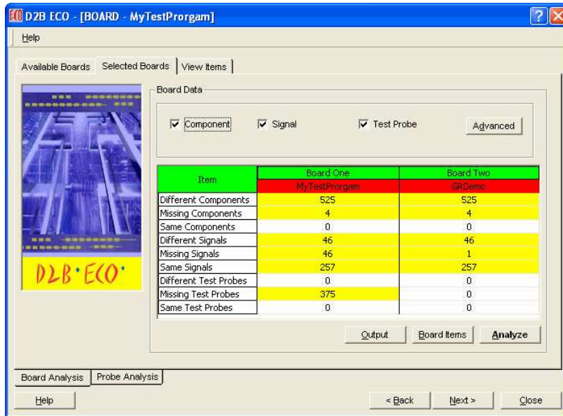
D2B ECO allows users to compare two revisions of a PCB assembly, performing checks for added, removed, or modified components
