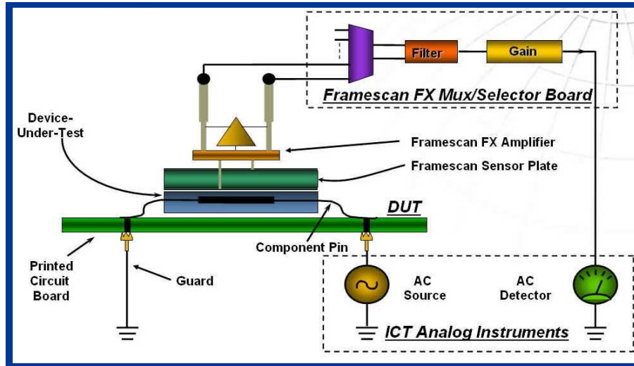
Block Diagram of Analog Framescan Test Technique
