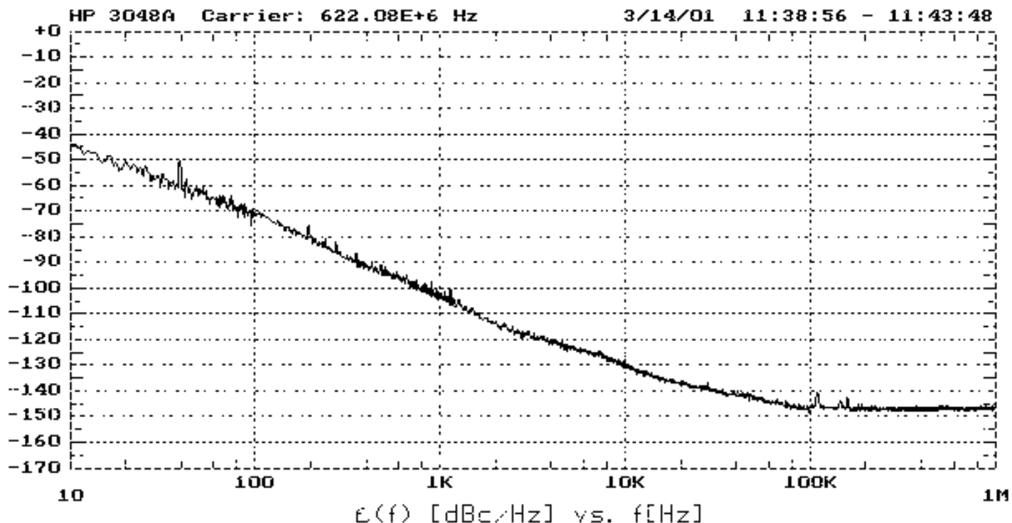
Single-Sideband Phase Noise
