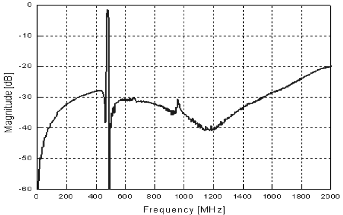
Passband Plot
