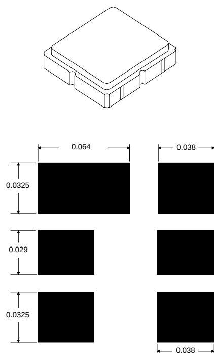
Foot Print Dimensions in Nominal Inches
