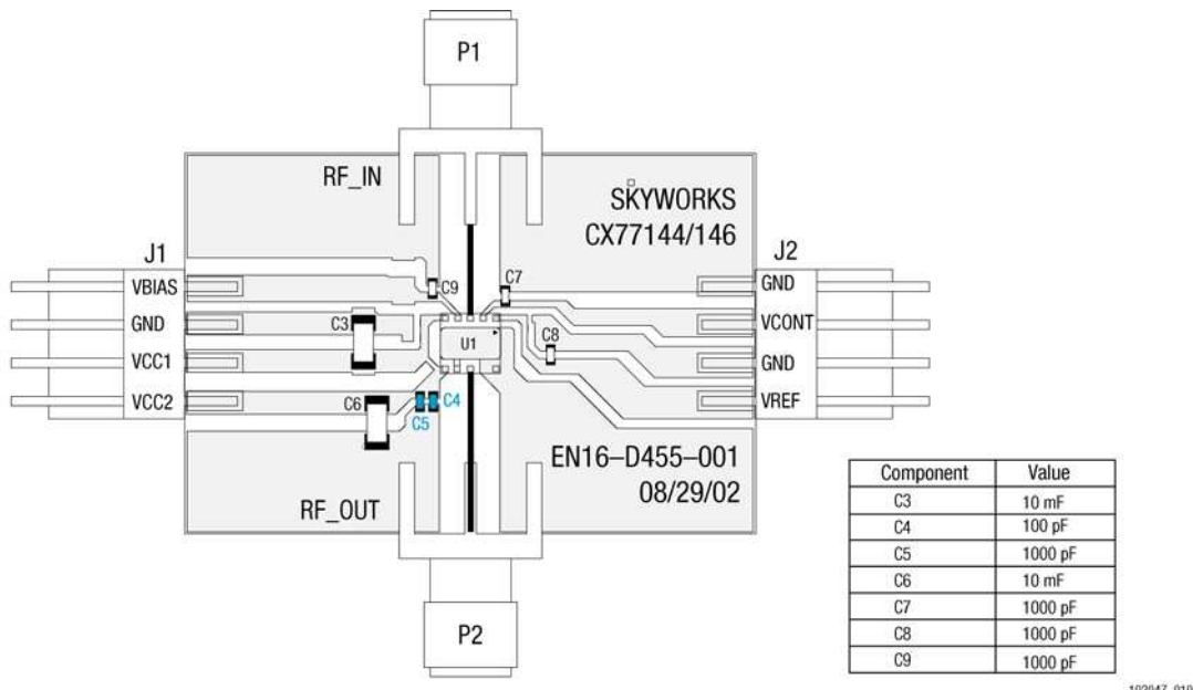
Figure 8. Evaluation Board Assembly Diagram
