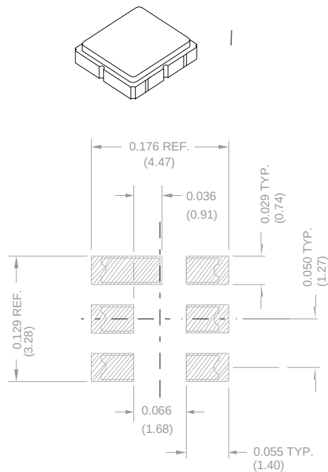
PCB Footprint
