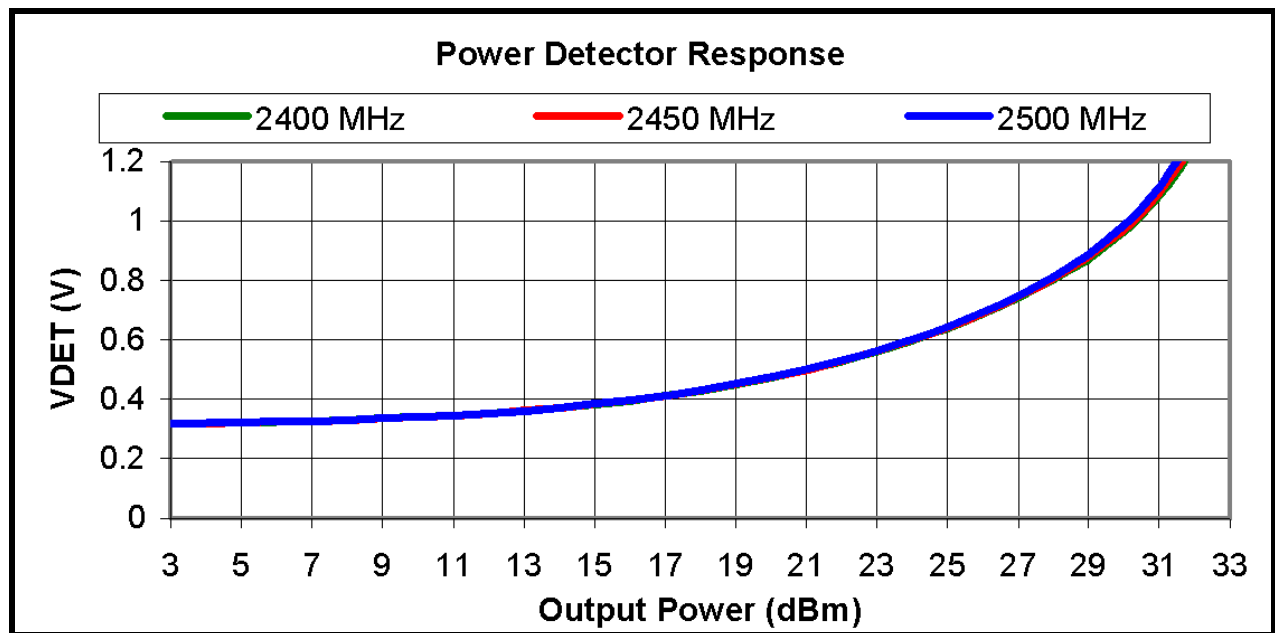
Figure 3: SE2605L Detector Characteristics
