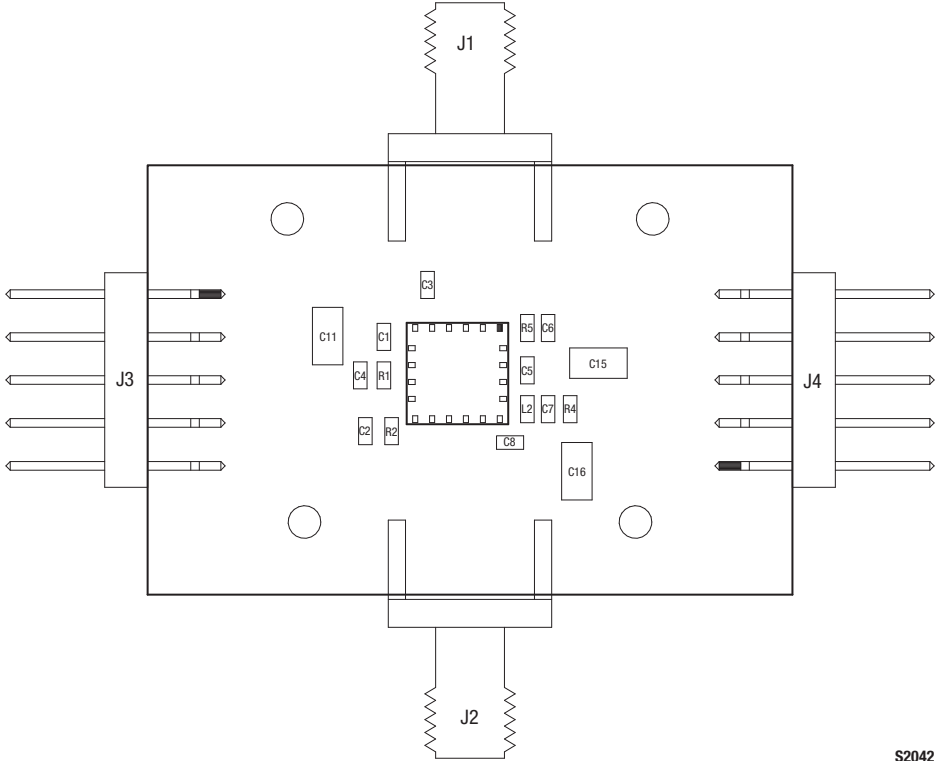
Figure 9. SKY65170-21 Evaluation Board Assembly Drawing
