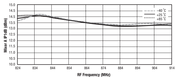
Figure 20. Mixer A Input P1dB vs Frequency and Temperature
