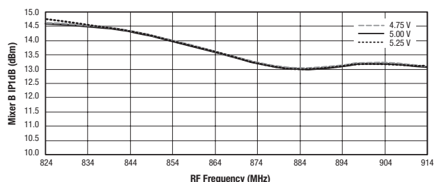
Figure 22. Mixer B Input P1dB vs Frequency and Supply Voltage
