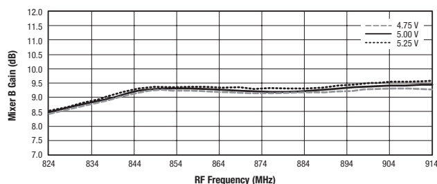
Figure 6. Mixer B Gain vs Frequency and Supply Voltage
