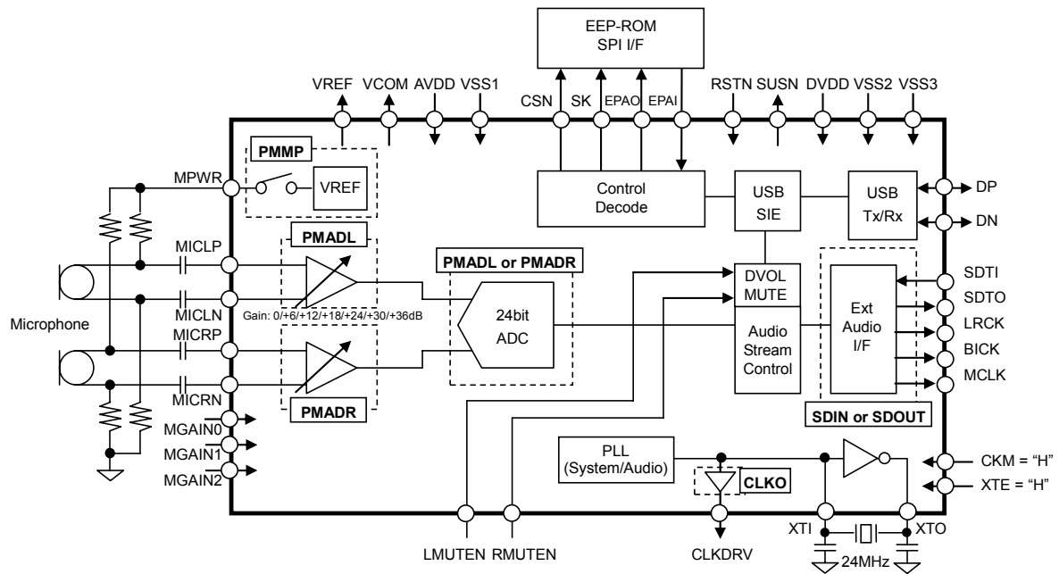
Figure 1. Block Diagram
