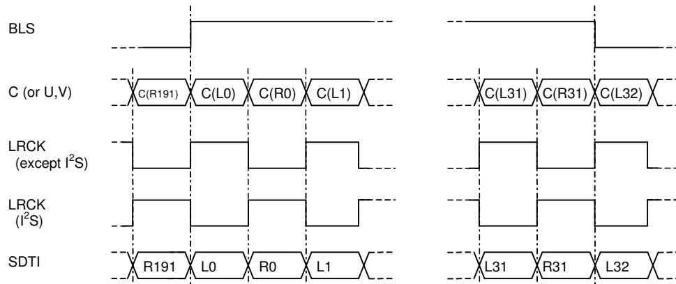
Figure 1. Audio routing mode timing (AKMODE pin = "0")
