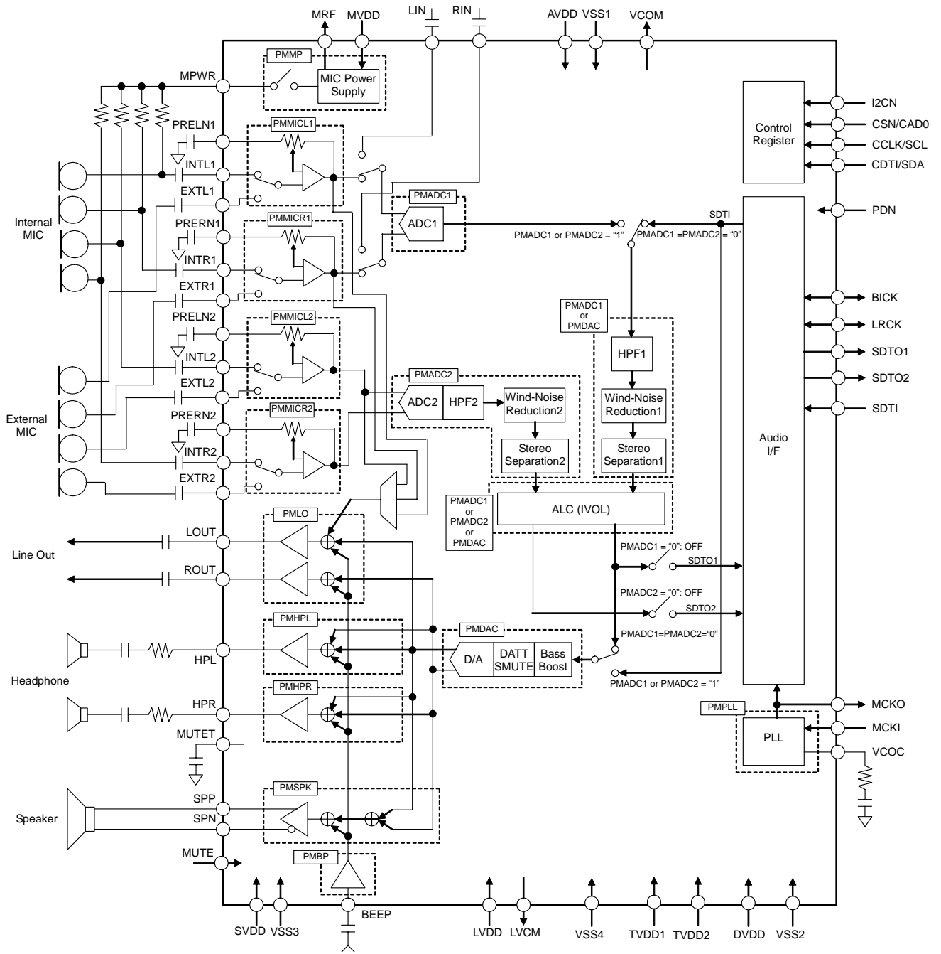
Figure 1. Block Diagram
