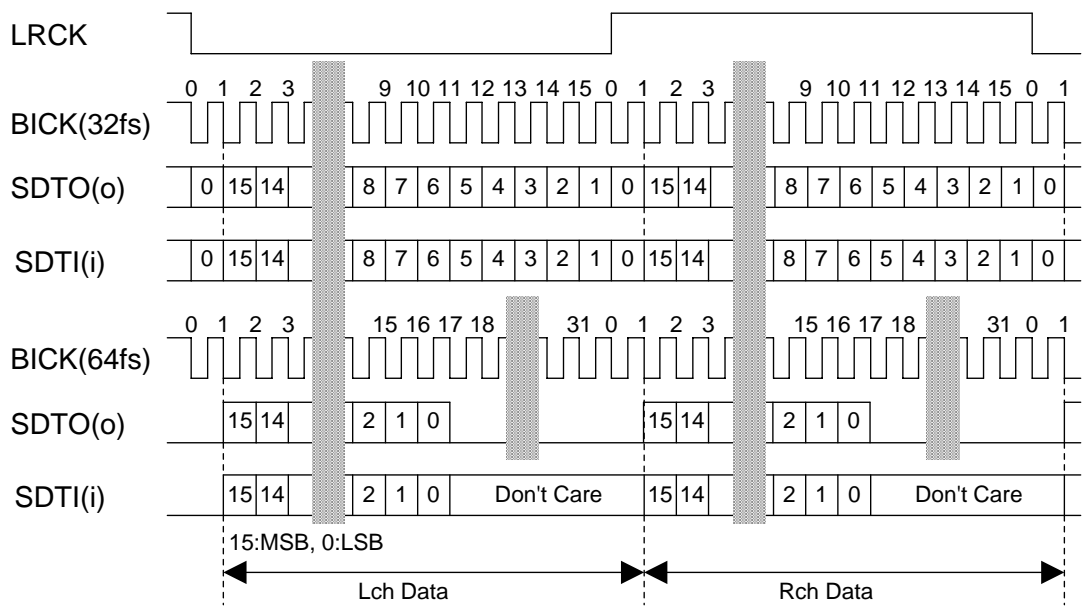
Figure 20. Mode 3 Timing
