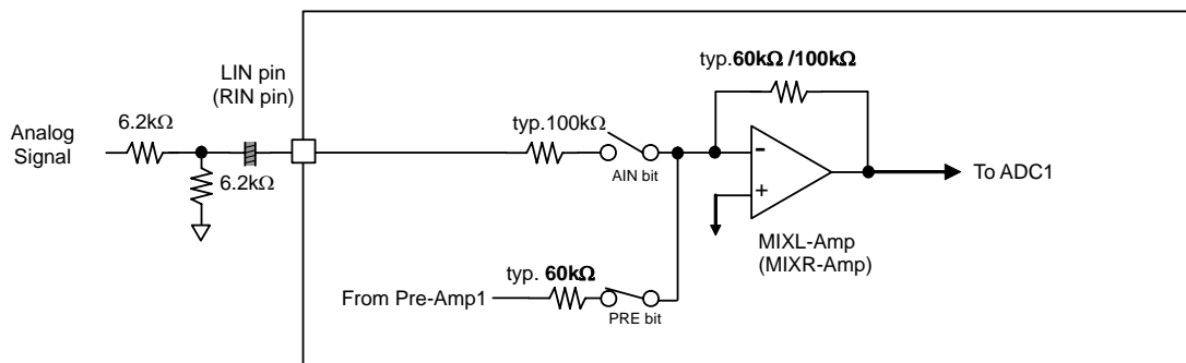
Figure 23. Analog Mixing Circuit for Recording Block
