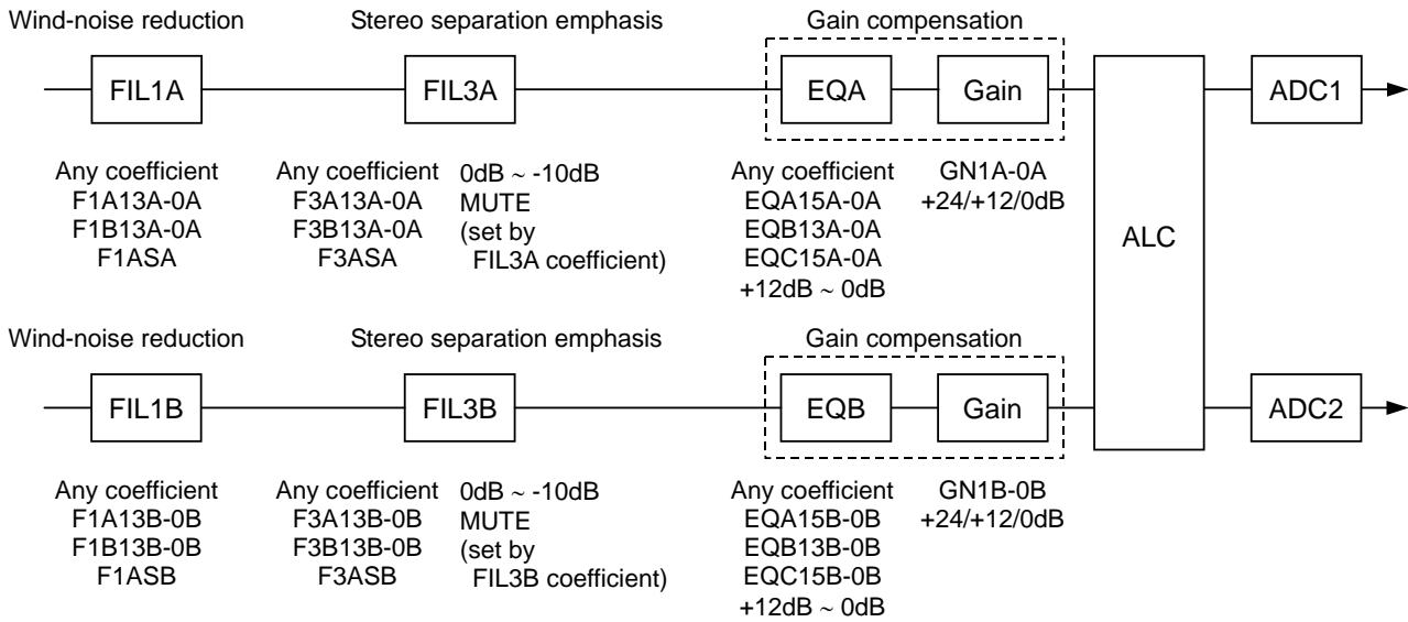
Figure 25. Digital EQ/HPF/LPF
