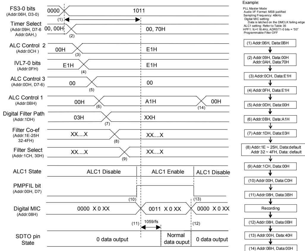
Figure 85. Digital MIC Input Recording Sequence
