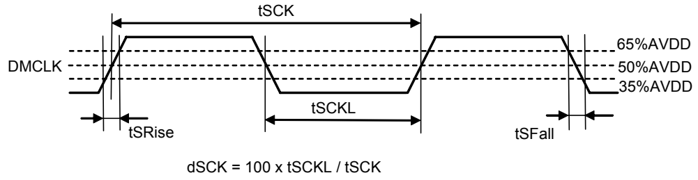
Figure 13. DMCLK Clock Timing
