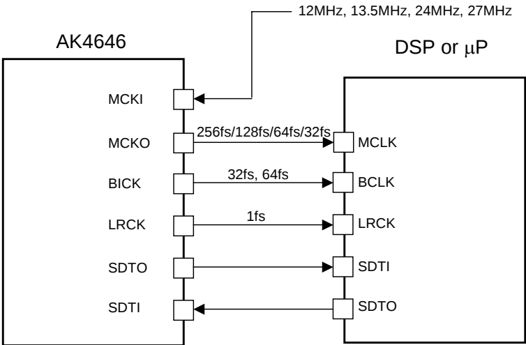
Figure 12. PLL Master Mode
