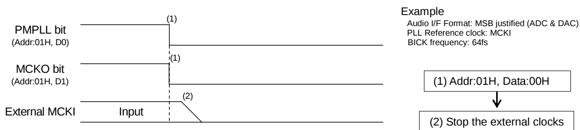
Figure 48. Clock Stopping Sequence (3)
