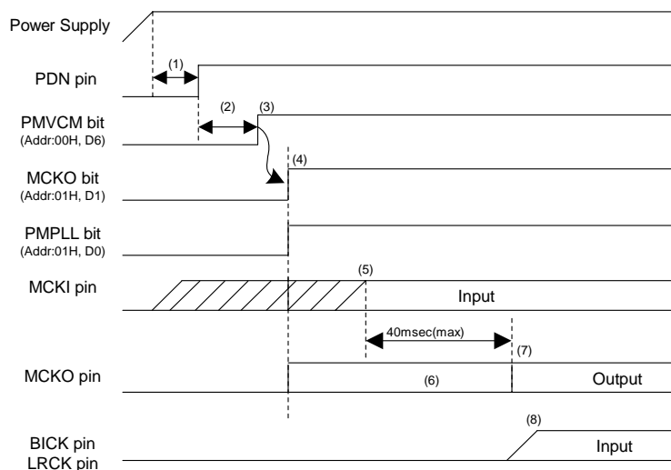
Figure 77. Clock Set Up Sequence (3)
