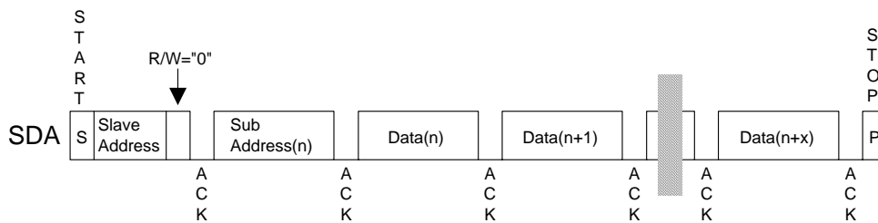
Figure 62. Data Transfer Sequence at the I 2 C-Bus Mode
