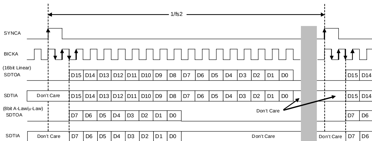
Figure 80. Timing of Short Frame Sync (PCM I/F A: MSBSA bit = "1", BCKPA bit = "1")
