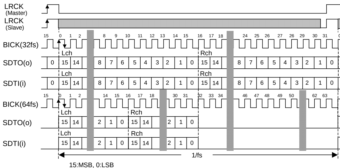
Figure 37. Mode 0 Timing (BCKP bit = "0", MSBS bit = "1")
