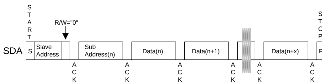
Figure 97. Data Transfer Sequence at the I 2 C-Bus Mode
