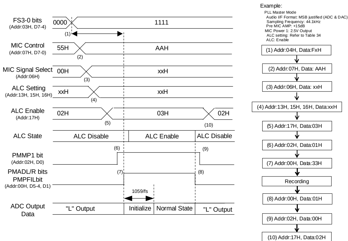
Figure 113. Stereo MIC Input Sequence (MIC Recording: LINx/RINx → MICL/R → ADCL/R → ALC → Audio I/F → SDTO)
