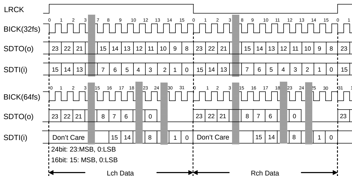
Figure 39. Mode 1 Timing
