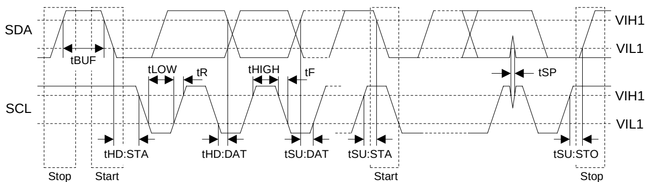
Figure 25. I²C Bus Mode Timing
