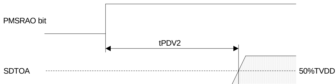
Figure 28. Power Down &amp; Reset Timing 3
