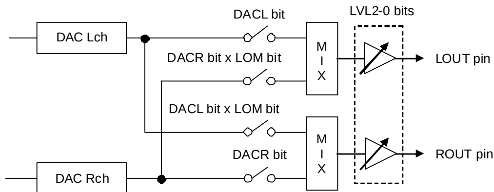
Figure 66. Stereo Line Output
