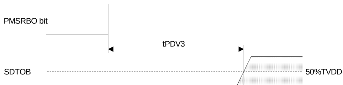
Figure 29. Power Down &amp; Reset Timing 4
