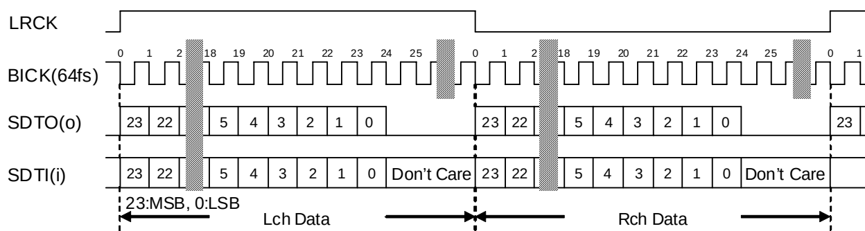
Figure 40. Mode 2 Timing
