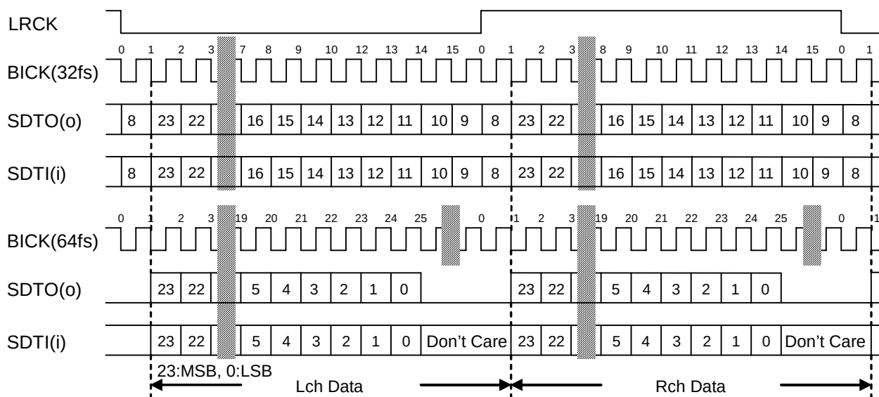
Figure 41. Mode 3 Timing
