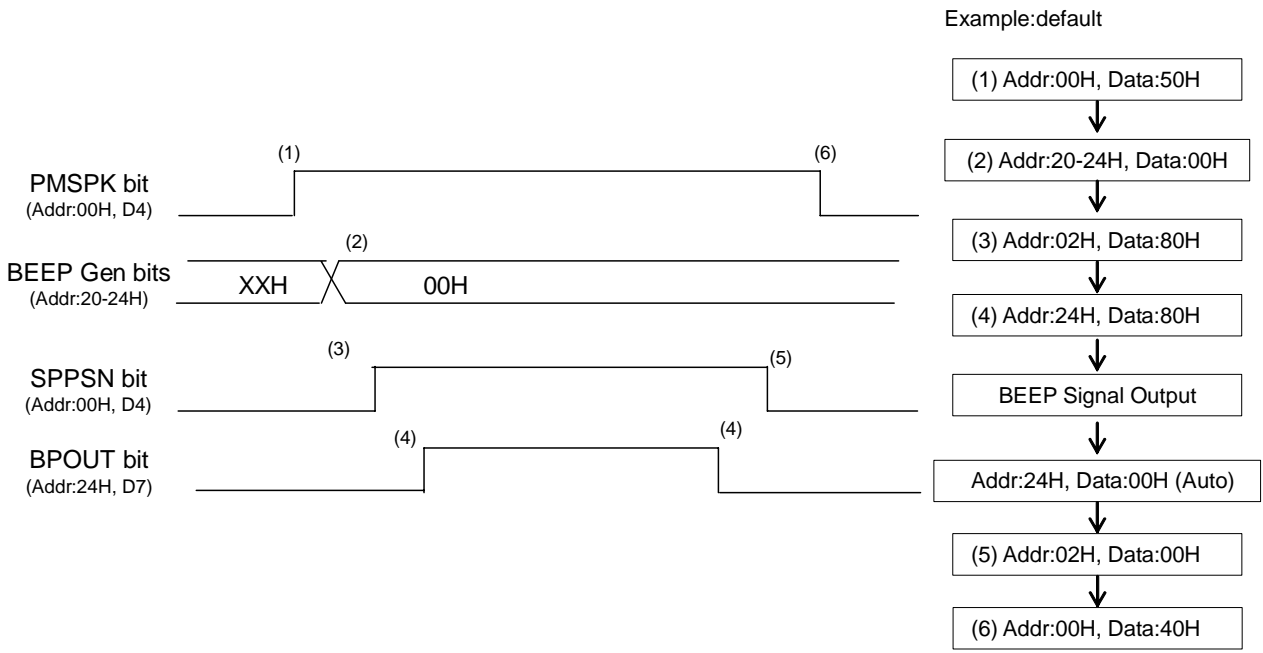
Figure 78. “BEPP Generator → Speaker-Amp” Output Sequence
