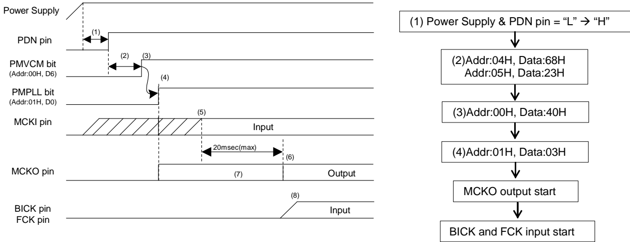
Figure 72. Clock Set Up Sequence (3)
