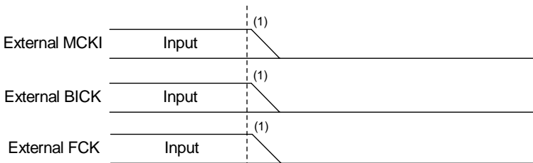
Figure 83. Clock Stopping Sequence (4)
