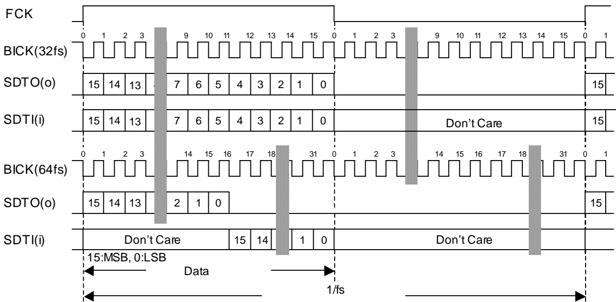
Figure 30. Mode 1 Timing
