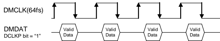
Figure 41. Data In/Output Timing with Digital MIC (DCLKP bit = “1”)
