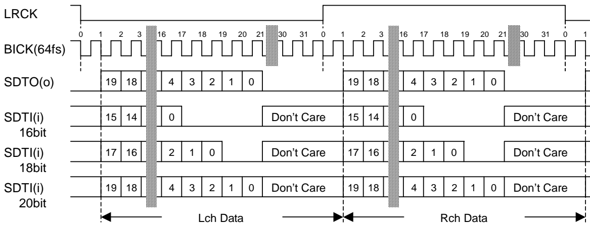
Figure 11. Mode 3 Timing
