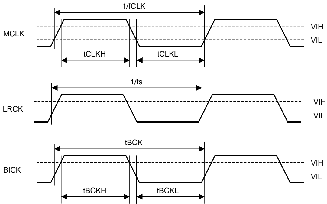
Figure 5. Clock Timing
