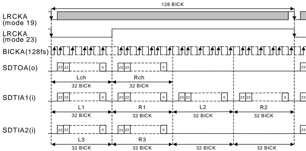
Figure 19. Mode 19 ,23 Timing
