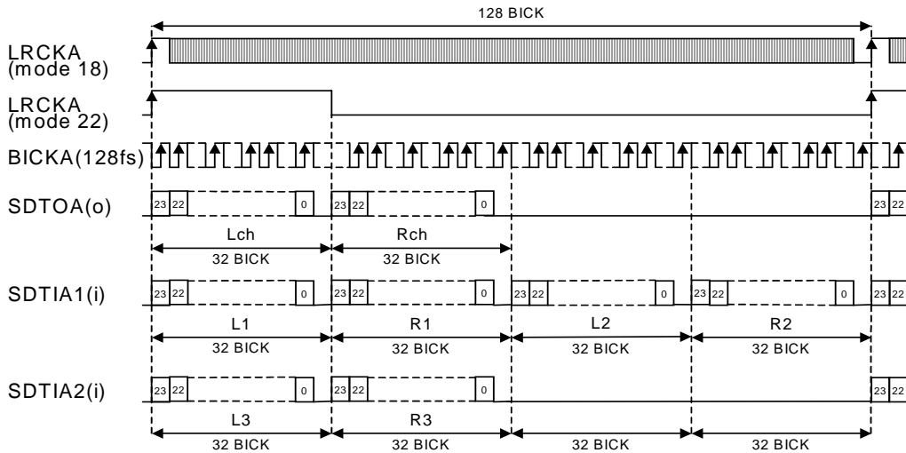
Figure 18. Mode 18 ,22 Timing
