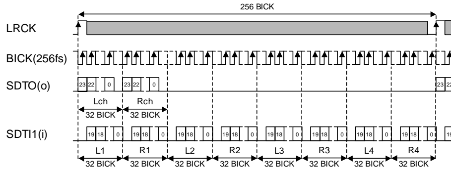
Figure 5. Mode 4 Timing
