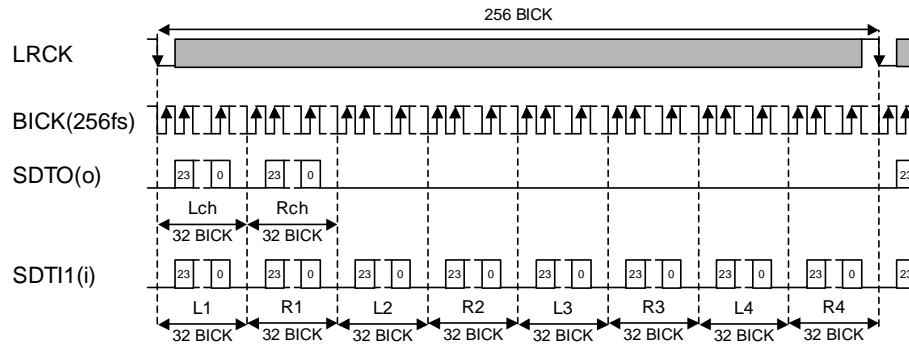
Figure 8. Mode 7 Timing
