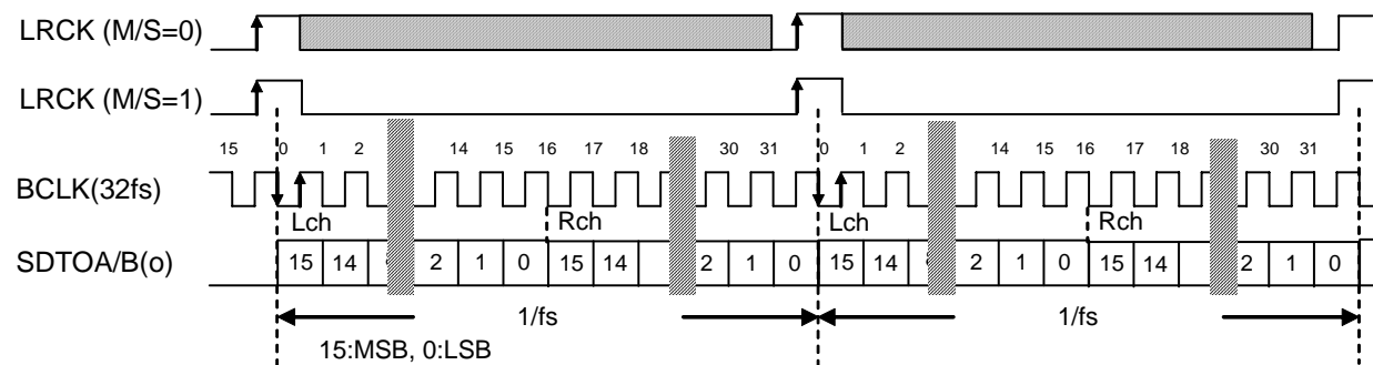
Figure 26. Mode 0, 4 Timing (Stereo Mode, DSP Mode 0, MSBS = "0", BCKP = "1")
