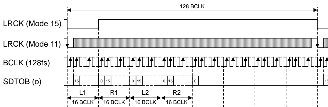
Figure 32. Mode 11, 15 Timing (TDM128 mode, I²S compatible)
