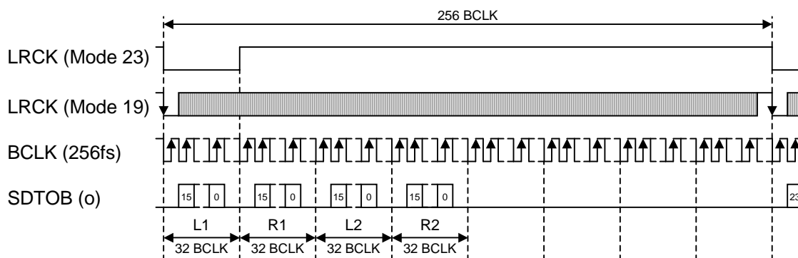
Figure 34. Mode 19, 23 Timing (TDM256 mode, I²S compatible)
