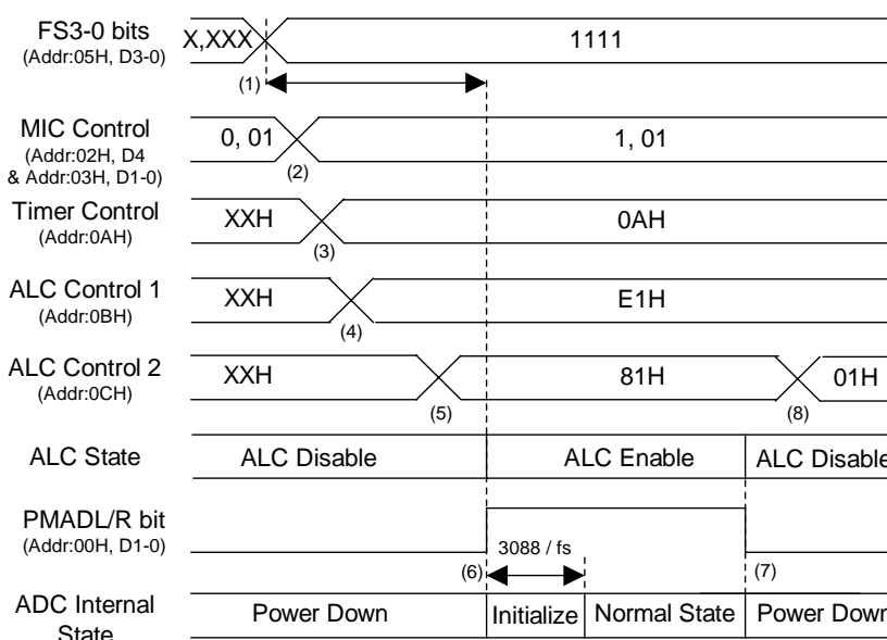
Figure 64. MIC Input Recording Sequence
