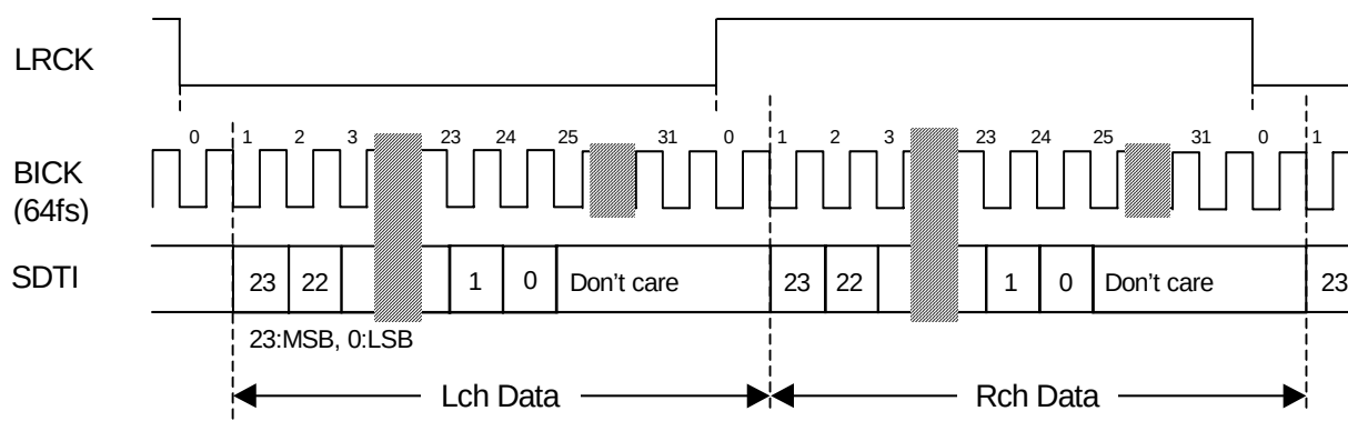
Figure 9. Mode 3 Timing
