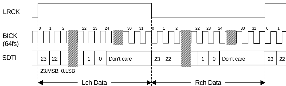
Figure 8. Mode 2 Timing
