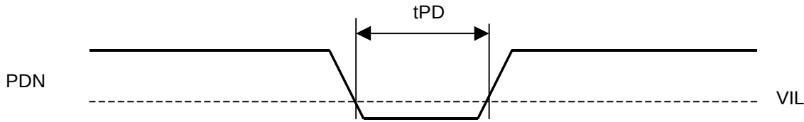
Figure 5. Power-down Timing
