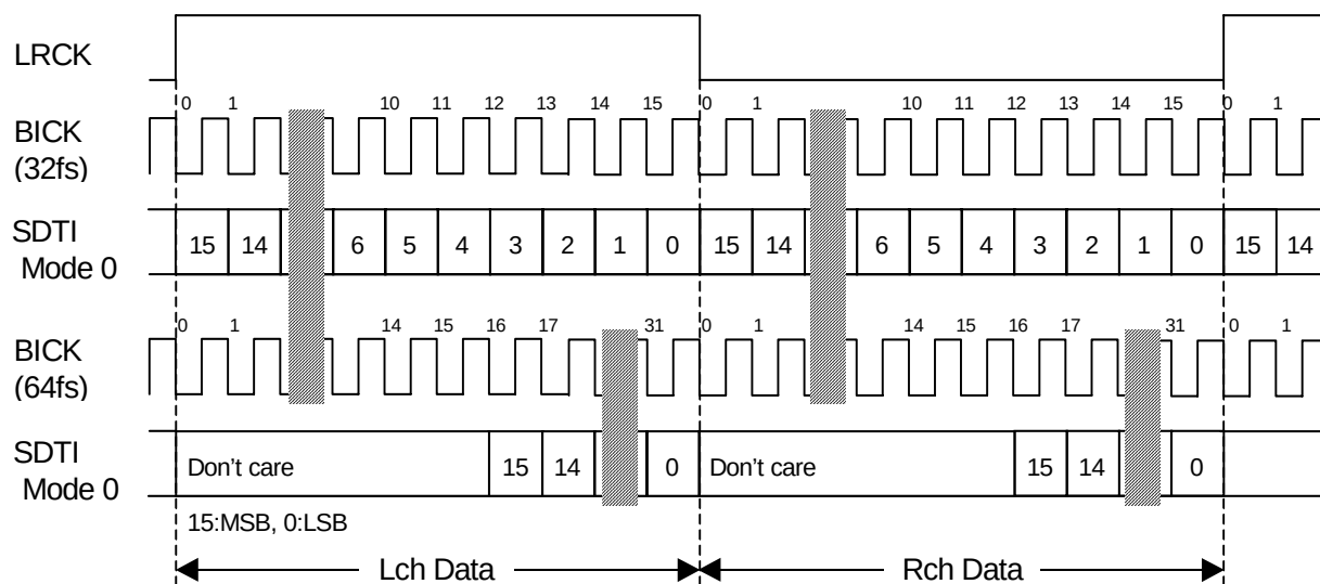
Figure 6. Mode 0 Timing
