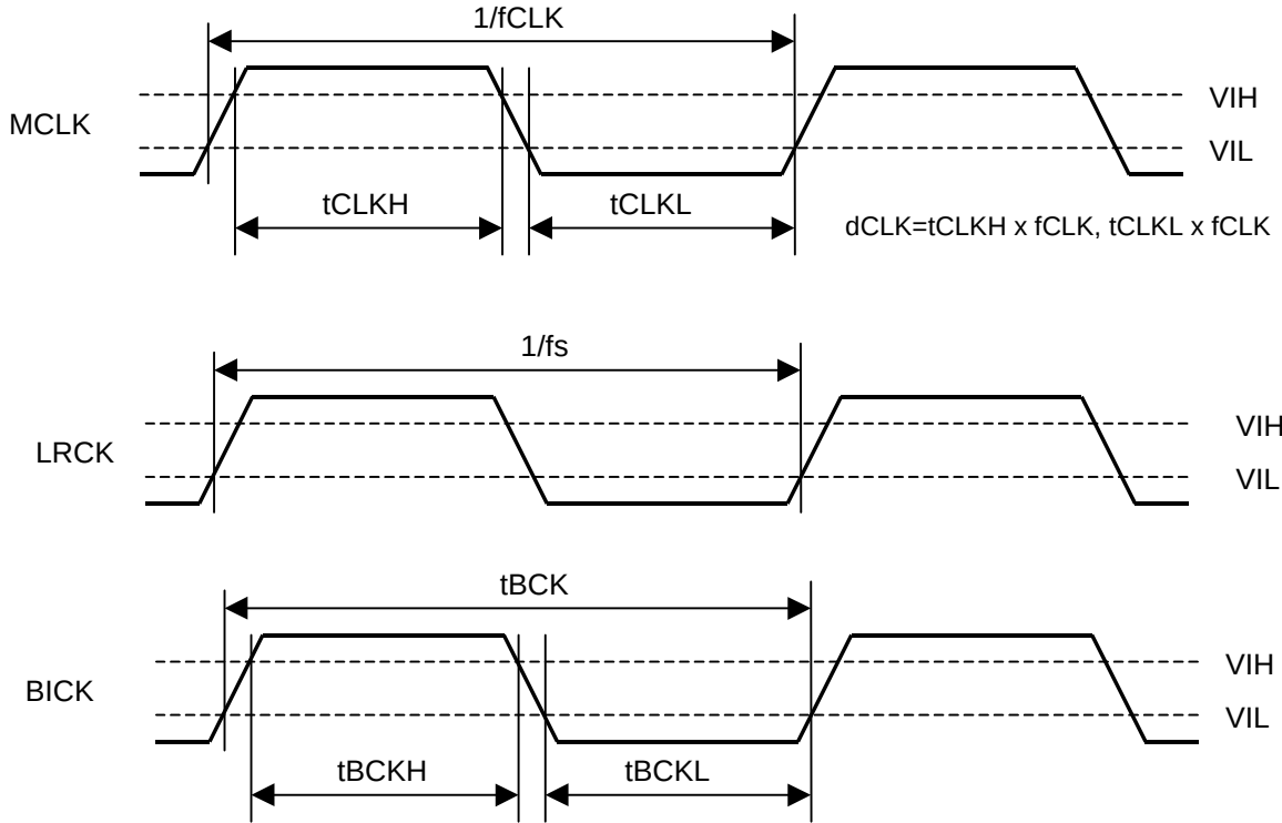
Figure 1. Clock Timing
