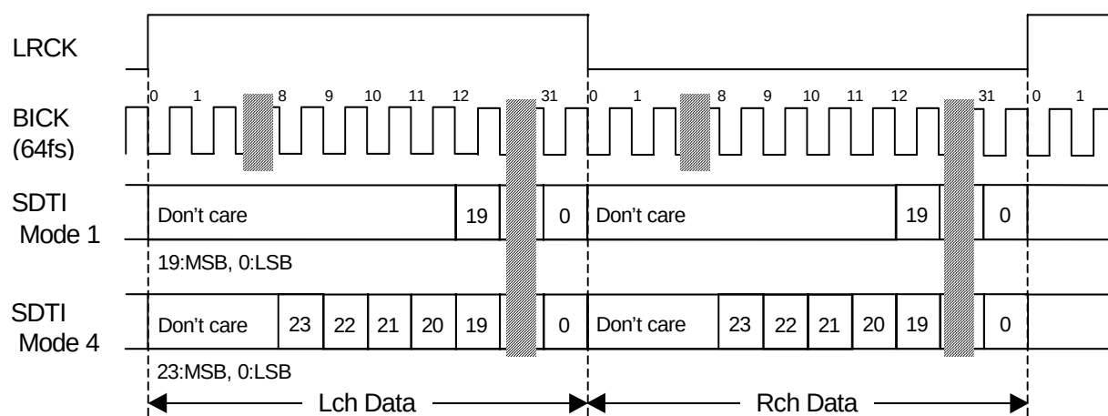
Figure 7. Mode 1,4 Timing
