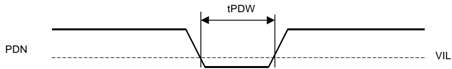
Power-down &amp; Reset Timing
