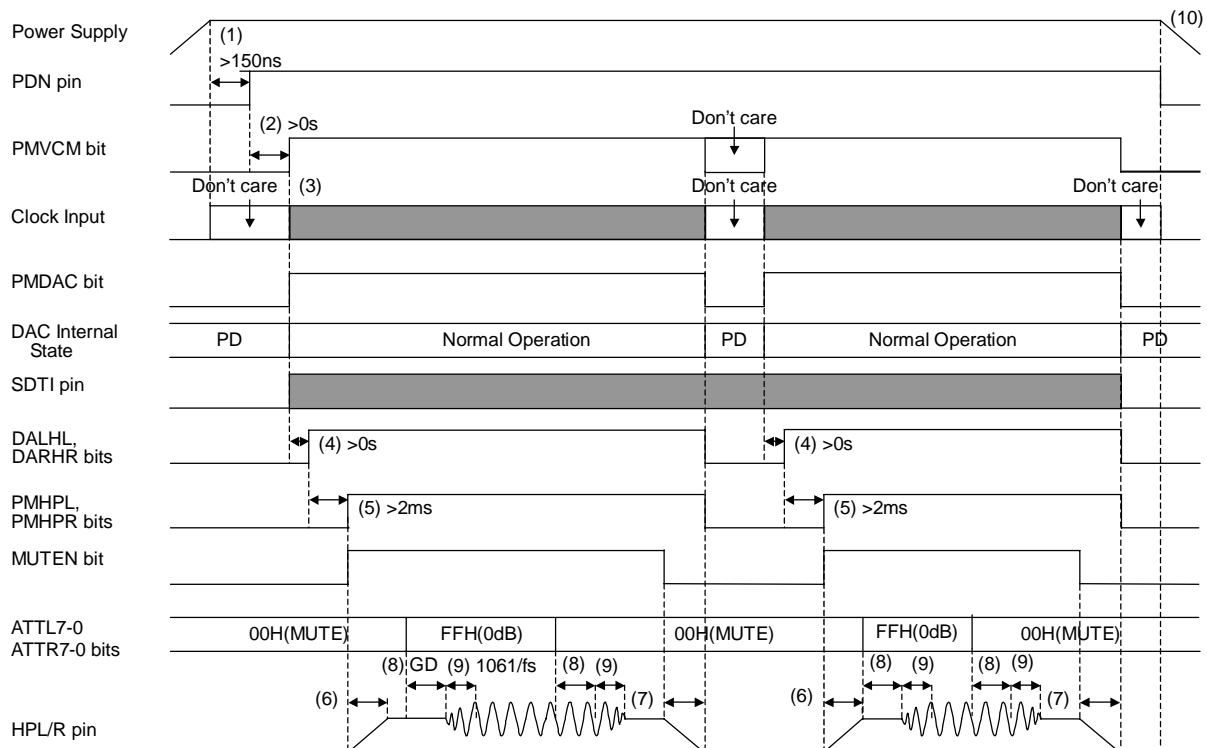
Figure 28. Power-up/down sequence of DAC and HP-amp (Don't care: except Hi-Z)
