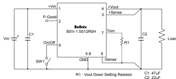
<Standard Connection Diagram>
