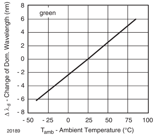
Figure 12. Change of Dominant Wavelength vs. Ambient Temperature
