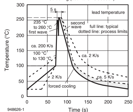
Figure 20. Double Wave Soldering of Opto Devices (all Packages)
