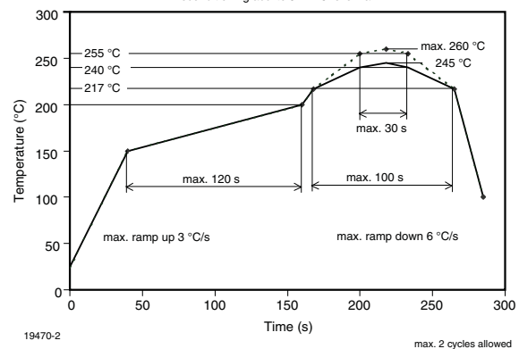
Figure 19. Vishay Lead (Pb)-free Reflow Soldering Profile (acc. to J-STD-020)
