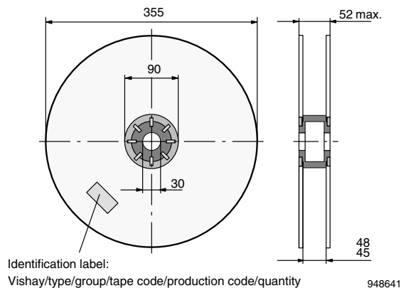
Figure 24. Reel Dimensions
