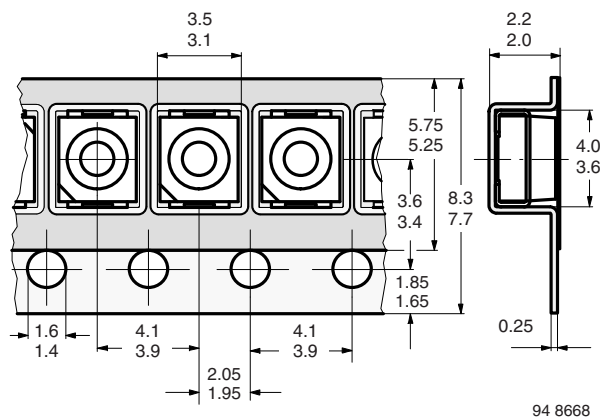
Fig. 23 - Tape Dimensions in mm for PLCC-2
