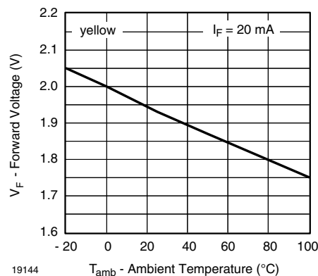
Figure 12. Forward Voltage vs. Ambient Temperature
