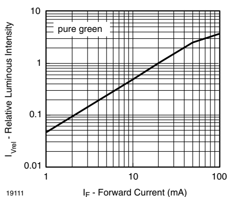
Fig. 18 - Relative Luminous Intensity vs. Forward Current
