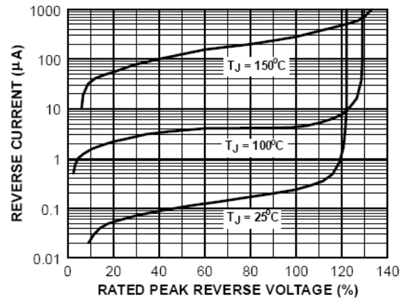
Figure 4. Reverse Characteristics
