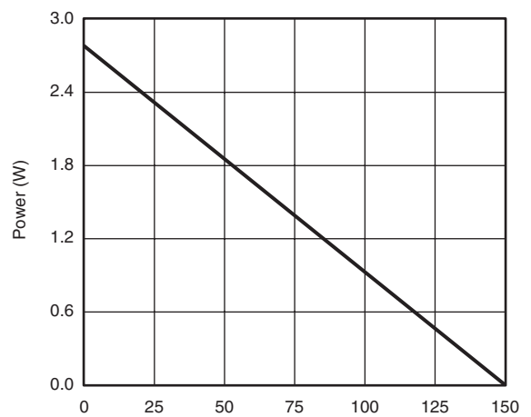
Power, Junction-to-Ambient
