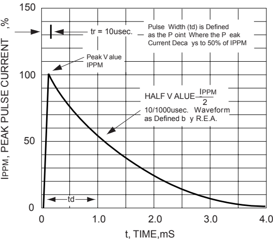
FIG. 3 - PULSE WAVEFORM
