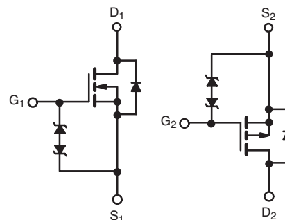
N-Channel MOSFET
