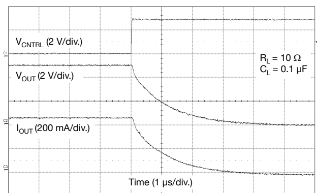
Figure 27 - SiP32413 Channel 1 Turn-Off (V IN = 5 V, R L = 10 Ω)
