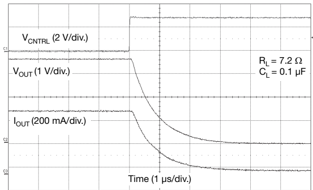
Figure 25 - SiP32413 Channel 1 Turn-Off (V IN = 3.6 V, R L = 7.2 Ω)
