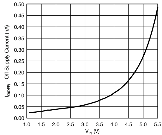
Figure 4 - Off Supply Current vs. Input Voltage
