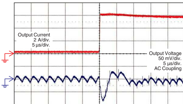
Transient Response in Continuous Conduction Mode ( 0.2 A - 6 A ) ( V_{IN} = 12\text{ V} , V_{OUT} = 1\text{ V} , FSW = 500\text{ kHz} )
