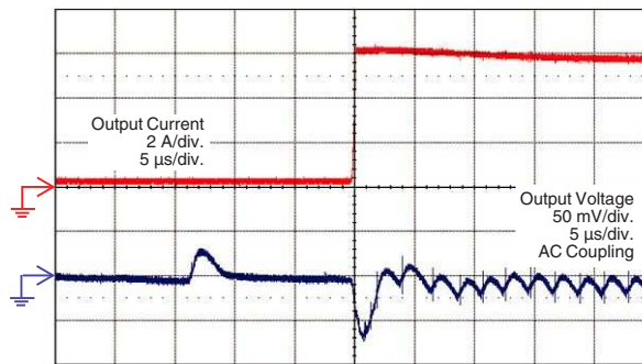
Transient Response in Power Save Mode ( 0.2 A - 6 A ) ( V_{IN} = 12\text{ V} , V_{OUT} = 1\text{ V} , FSW = 500\text{ kHz} at 6A)
