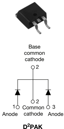
VS-15CTQ...SPbF
