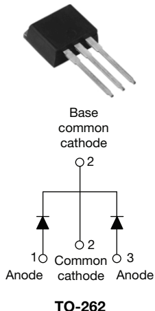
VS-15CTQ...-1PbF
