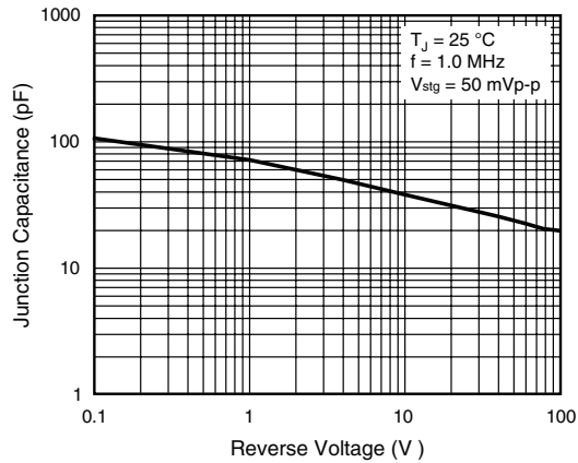
Figure 4. Typical Junction Capacitance Per Diode
