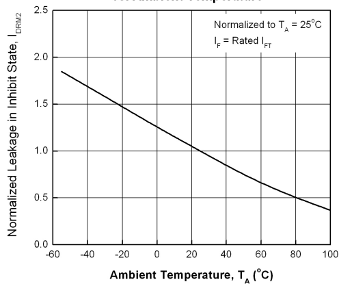
Figure 8. Leakage in Inhibit State vs. Ambient Temperature
