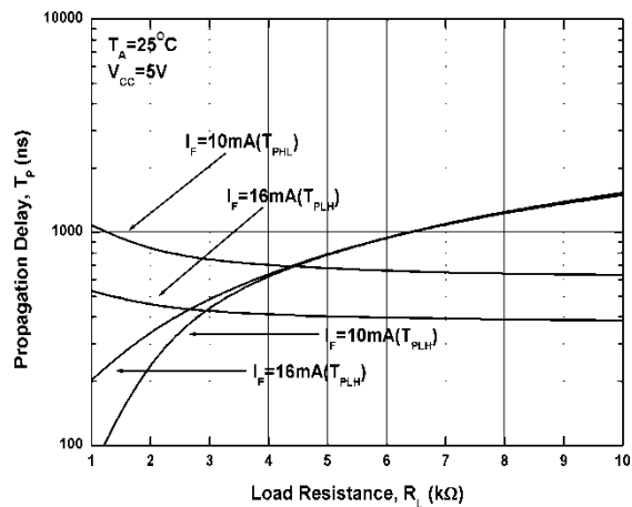
Figure 6. Propagation Delay vs. Load Resistance
