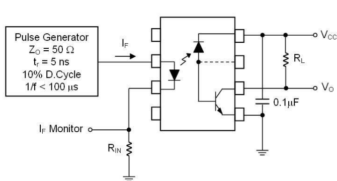
Figure 8 Switching Time Test Circuit & Waveform
