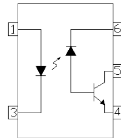
Pin Configuration
